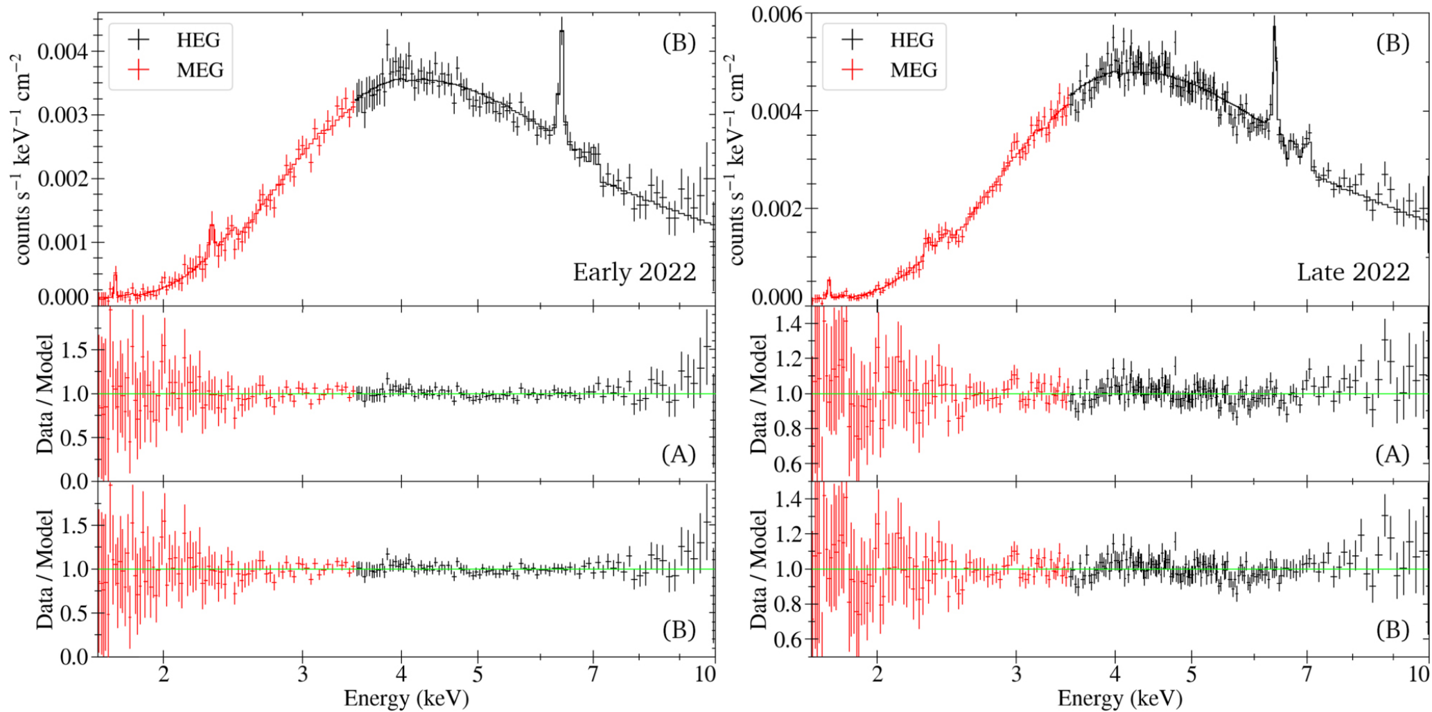
Figure 8. from David Bogensberger et al 2024 Astrophys. J. 961 doi:10.3847/1538-4357/ad1107 https://dx.doi.org/10.3847/1538-4357/ad1107 © 2024. The Author(s). Published by the American Astronomical Society.
