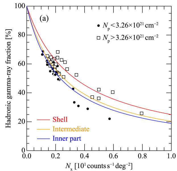
Figure 9. from Yasuo Fukui et al 2024 Astrophys. J. 961 doi:10.3847/1538-4357/ad0da3 https://dx.doi.org/10.3847/1538-4357/ad0da3 © 2024. The Author(s). Published by the American Astronomical Society.
