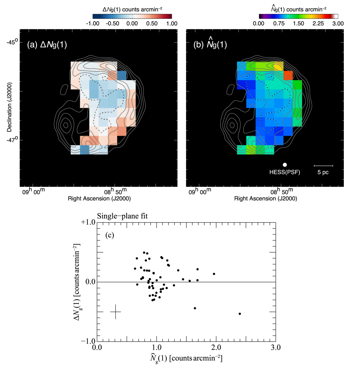
Figure 6. from Yasuo Fukui et al 2024 Astrophys. J. 961 doi:10.3847/1538-4357/ad0da3 https://dx.doi.org/10.3847/1538-4357/ad0da3 © 2024. The Author(s). Published by the American Astronomical Society.
