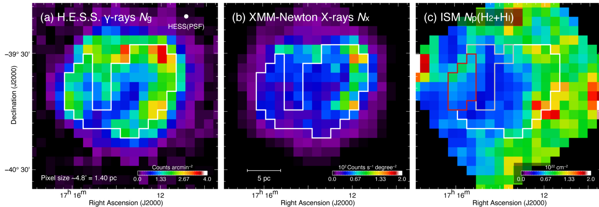
Figure 4. from Yasuo Fukui et al 2024 Astrophys. J. 961 doi:10.3847/1538-4357/ad0da3 https://dx.doi.org/10.3847/1538-4357/ad0da3 © 2024. The Author(s). Published by the American Astronomical Society.
