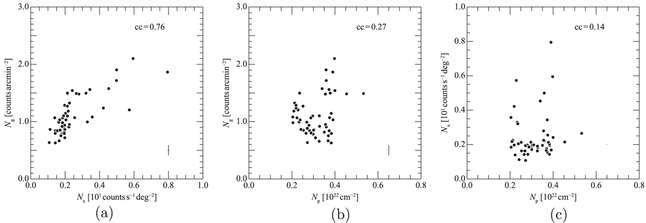
Figure 3. from Yasuo Fukui et al 2024 Astrophys. J. 961 doi:10.3847/1538-4357/ad0da3 https://dx.doi.org/10.3847/1538-4357/ad0da3 © 2024. The Author(s). Published by the American Astronomical Society.
