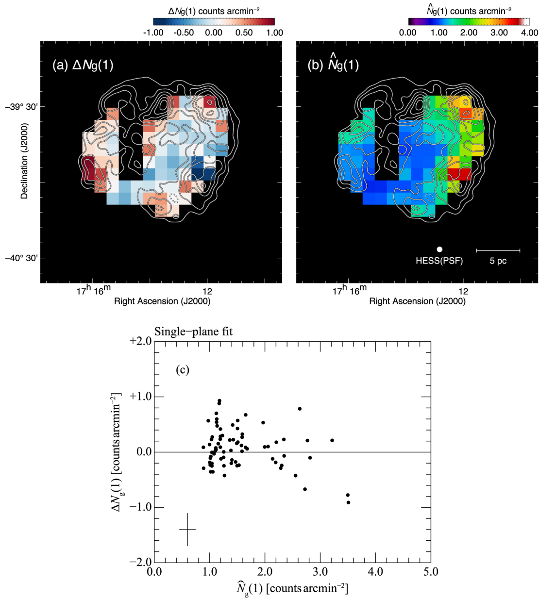
Figure 10. from Yasuo Fukui et al 2024 Astrophys. J. 961 doi:10.3847/1538-4357/ad0da3 https://dx.doi.org/10.3847/1538-4357/ad0da3 © 2024. The Author(s). Published by the American Astronomical Society.
