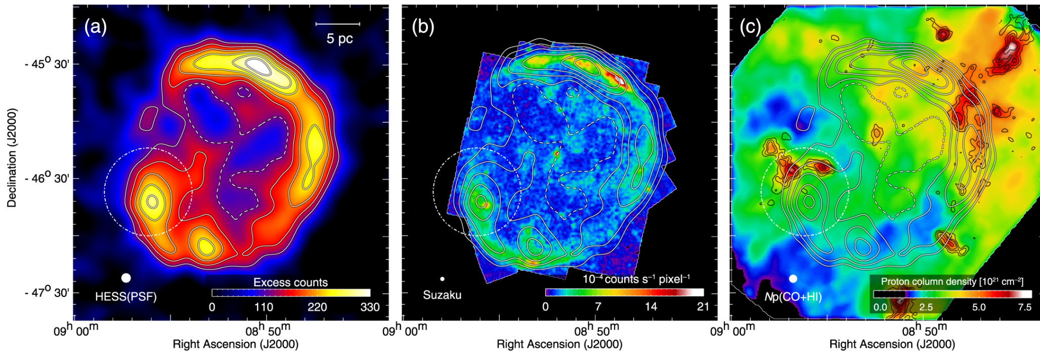
Figure 1. from Yasuo Fukui et al 2024 Astrophys. J. 961 doi:10.3847/1538-4357/ad0da3 https://dx.doi.org/10.3847/1538-4357/ad0da3 © 2024. The Author(s). Published by the American Astronomical Society.
