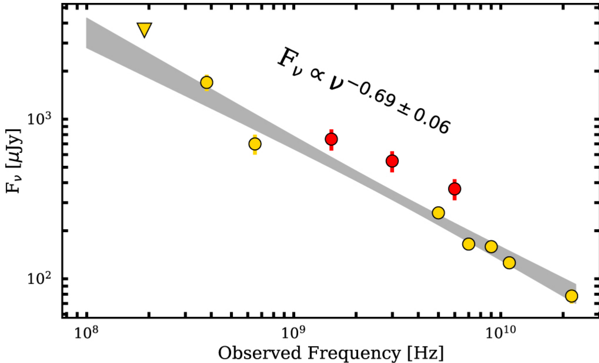
Figure 5. from Yuxin Dong et al 2024 Astrophys. J. 961 doi:10.3847/1538-4357/ad0cbd https://dx.doi.org/10.3847/1538-4357/ad0cbd © 2024. The Author(s). Published by the American Astronomical Society.
