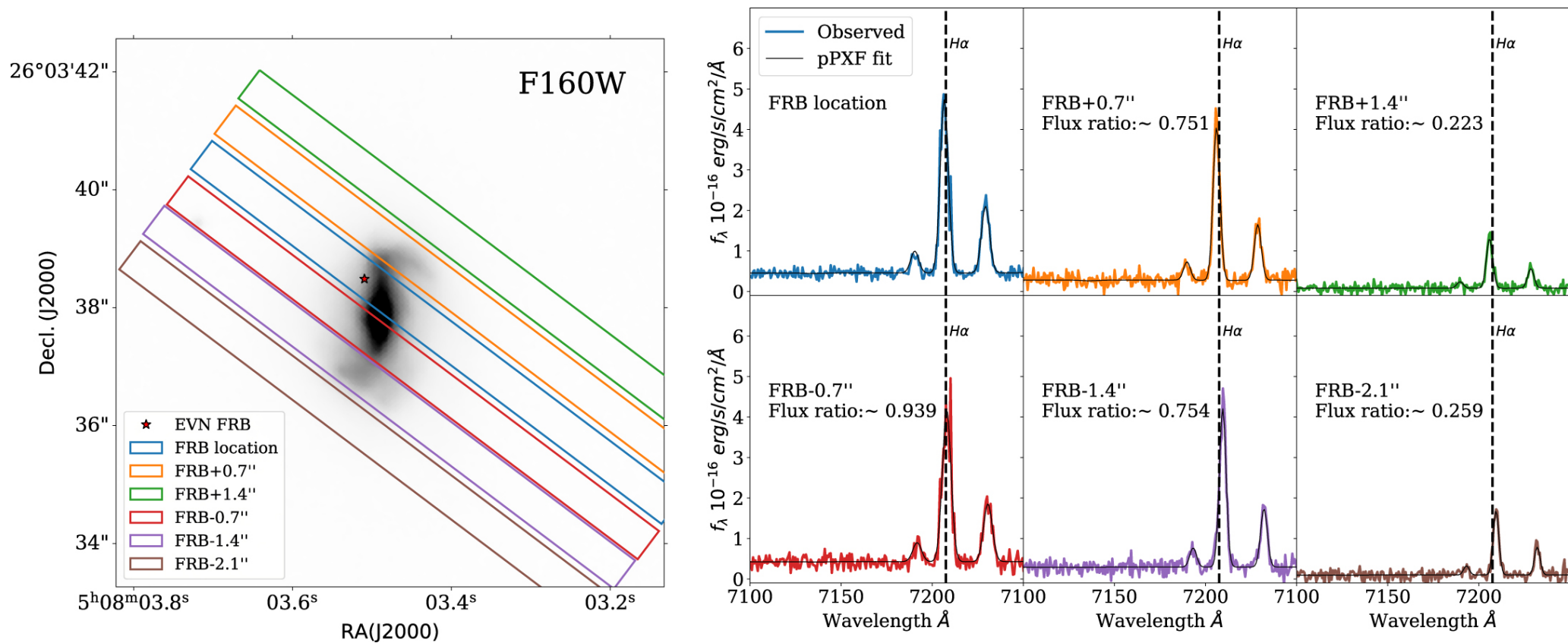
Figure 3. from Yuxin Dong et al 2024 Astrophys. J. 961 doi:10.3847/1538-4357/ad0cbd https://dx.doi.org/10.3847/1538-4357/ad0cbd © 2024. The Author(s). Published by the American Astronomical Society.
