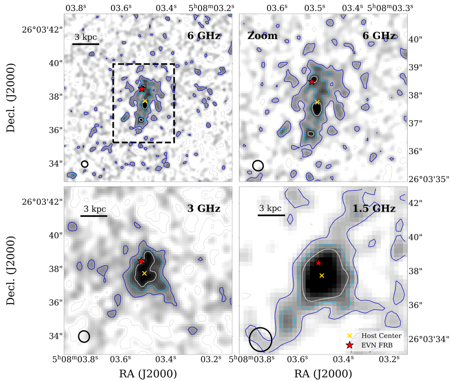
Figure 1. from Yuxin Dong et al 2024 Astrophys. J. 961 doi:10.3847/1538-4357/ad0cbd https://dx.doi.org/10.3847/1538-4357/ad0cbd © 2024. The Author(s). Published by the American Astronomical Society.
