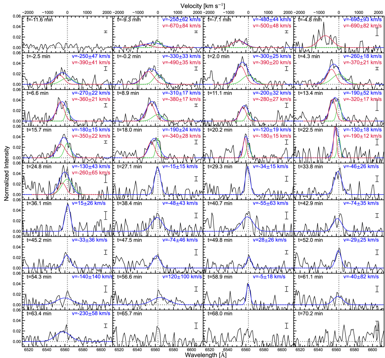
Figure 9. from Kosuke Namekata et al 2024 Astrophys. J. 961 doi:10.3847/1538-4357/ad0b7c https://dx.doi.org/10.3847/1538-4357/ad0b7c © 2024. The Author(s). Published by the American Astronomical Society.
