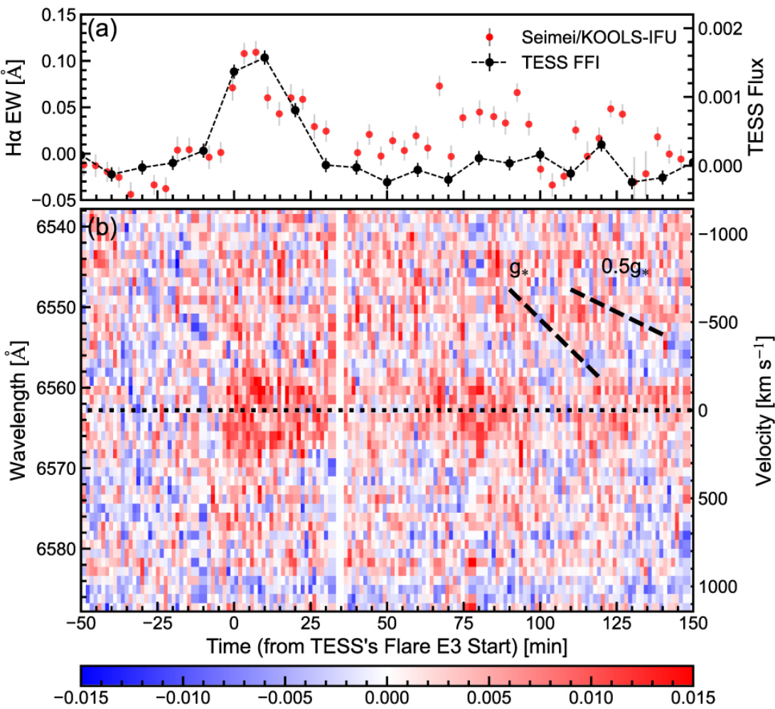
Figure 8. from Kosuke Namekata et al 2024 Astrophys. J. 961 doi:10.3847/1538-4357/ad0b7c https://dx.doi.org/10.3847/1538-4357/ad0b7c © 2024. The Author(s). Published by the American Astronomical Society.
