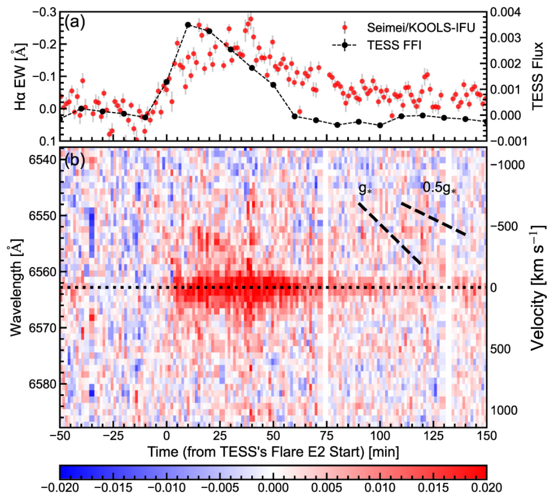
Figure 7. from Kosuke Namekata et al 2024 Astrophys. J. 961 doi:10.3847/1538-4357/ad0b7c https://dx.doi.org/10.3847/1538-4357/ad0b7c © 2024. The Author(s). Published by the American Astronomical Society.
