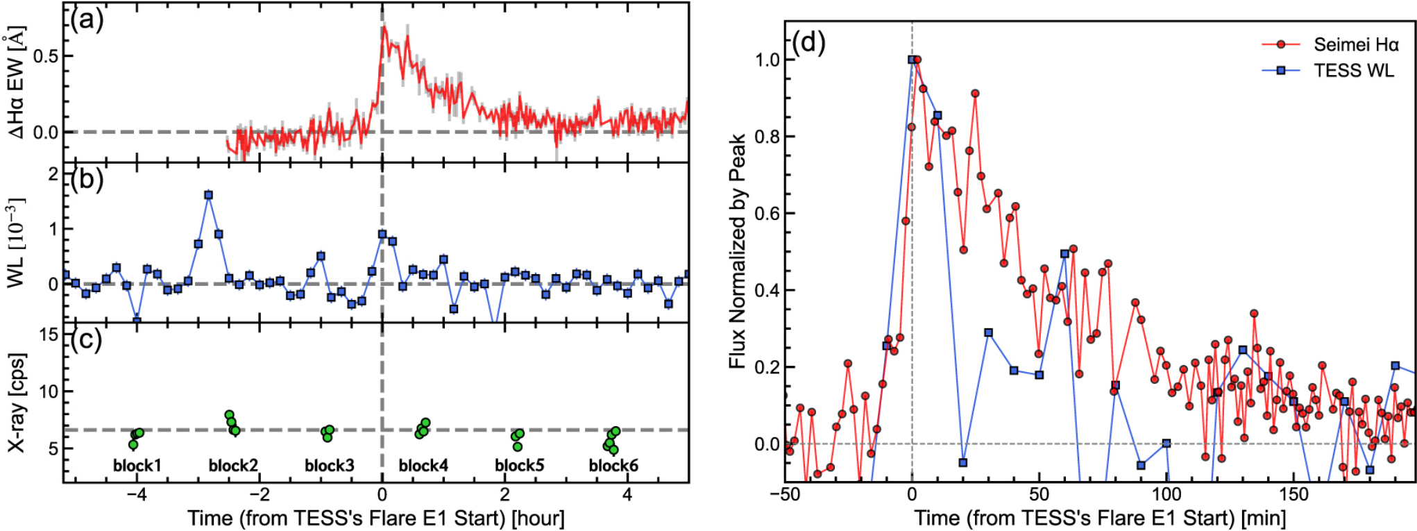
Figure 3. from Kosuke Namekata et al 2024 Astrophys. J. 961 doi:10.3847/1538-4357/ad0b7c https://dx.doi.org/10.3847/1538-4357/ad0b7c © 2024. The Author(s). Published by the American Astronomical Society.
