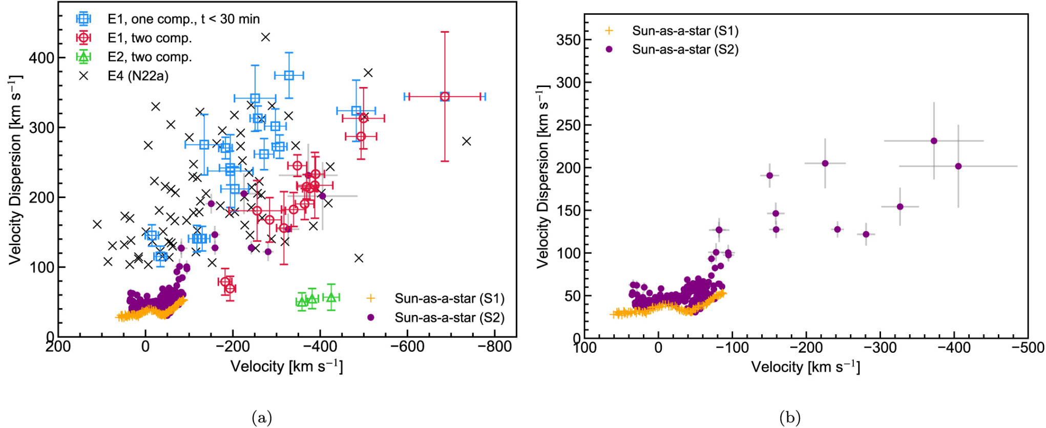
Figure 29. from Kosuke Namekata et al 2024 Astrophys. J. 961 doi:10.3847/1538-4357/ad0b7c https://dx.doi.org/10.3847/1538-4357/ad0b7c © 2024. The Author(s). Published by the American Astronomical Society.
