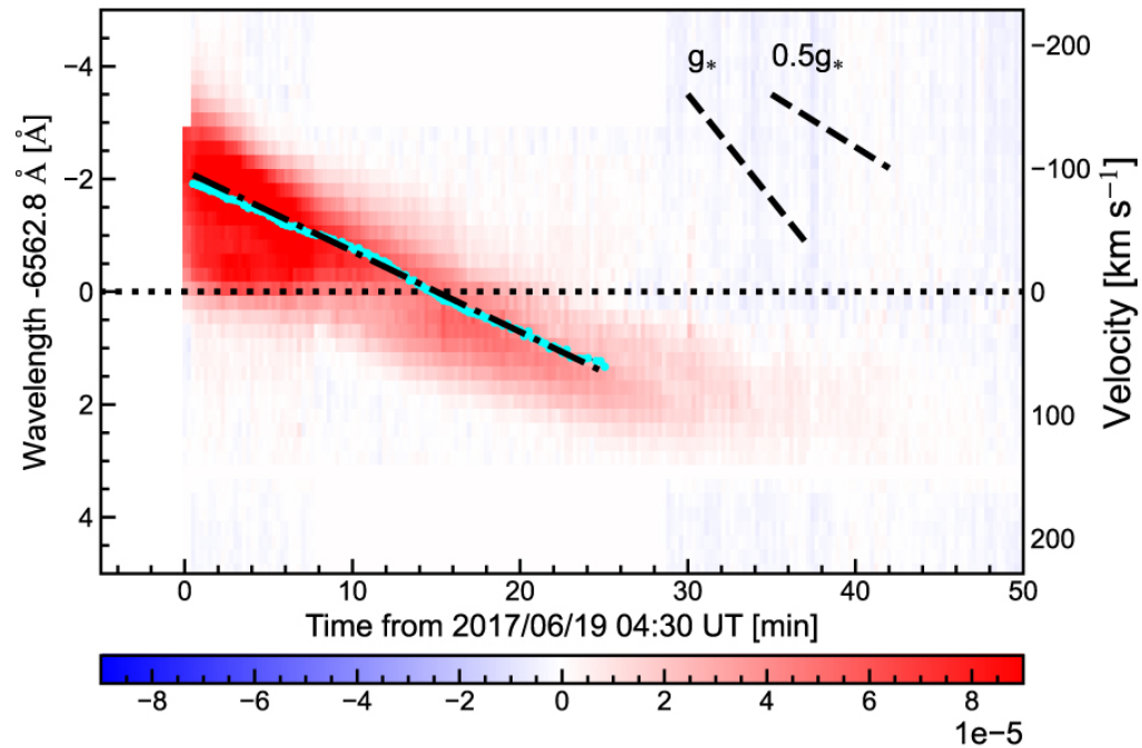
Figure 28. from Kosuke Namekata et al 2024 Astrophys. J. 961 doi:10.3847/1538-4357/ad0b7c https://dx.doi.org/10.3847/1538-4357/ad0b7c © 2024. The Author(s). Published by the American Astronomical Society.
