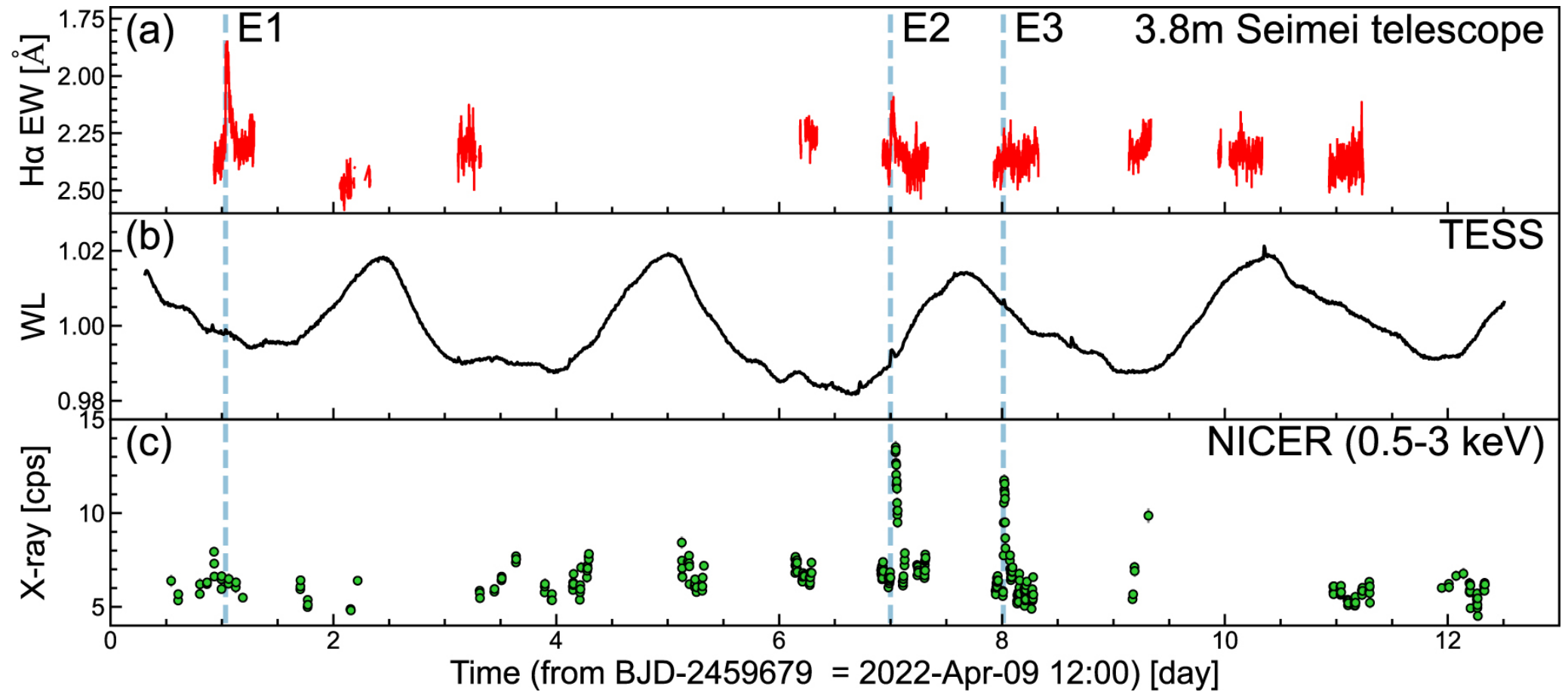
Figure 2. from Kosuke Namekata et al 2024 Astrophys. J. 961 doi:10.3847/1538-4357/ad0b7c https://dx.doi.org/10.3847/1538-4357/ad0b7c © 2024. The Author(s). Published by the American Astronomical Society.
