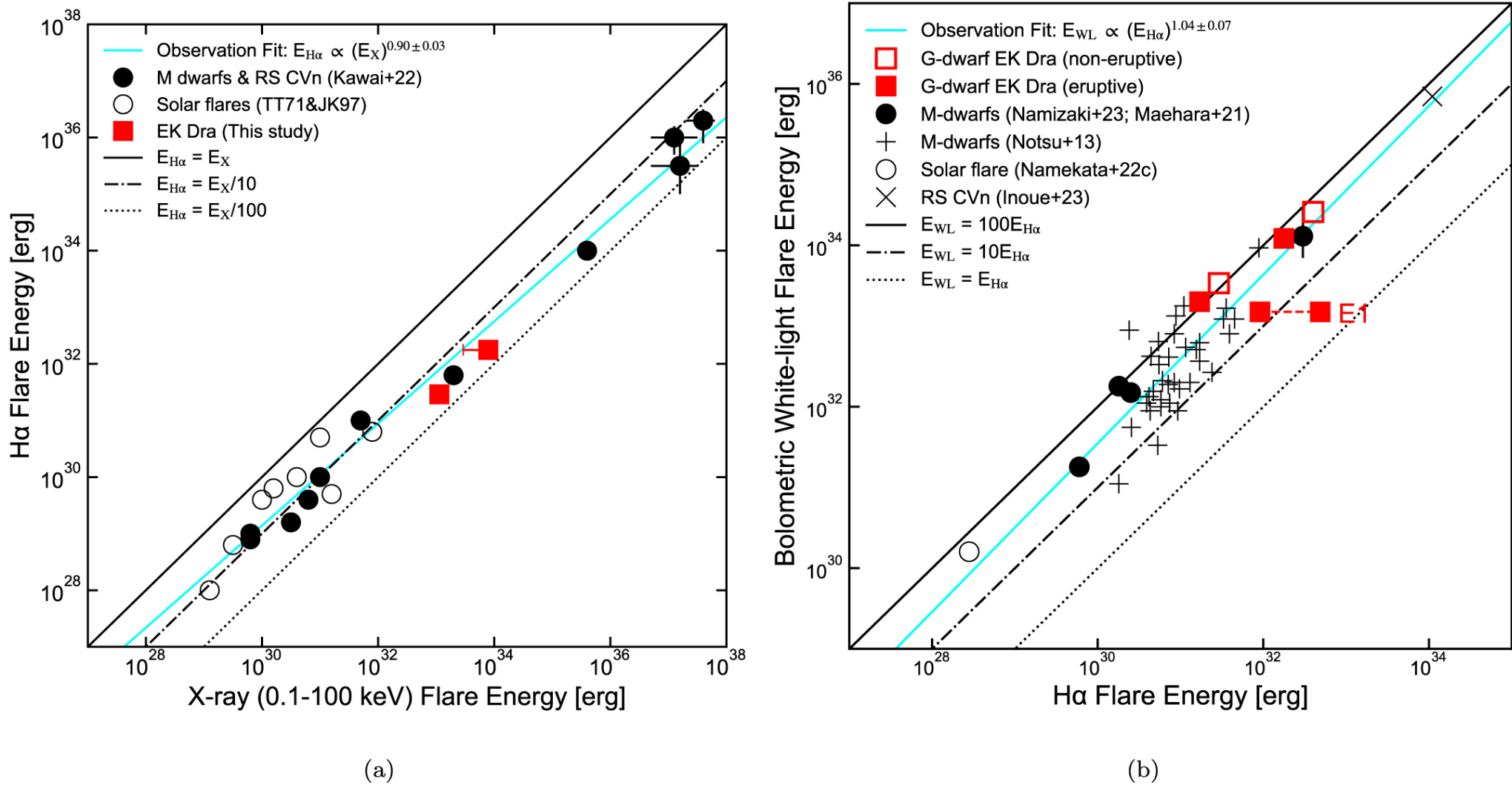
Figure 18. from Kosuke Namekata et al 2024 Astrophys. J. 961 doi:10.3847/1538-4357/ad0b7c https://dx.doi.org/10.3847/1538-4357/ad0b7c © 2024. The Author(s). Published by the American Astronomical Society.
