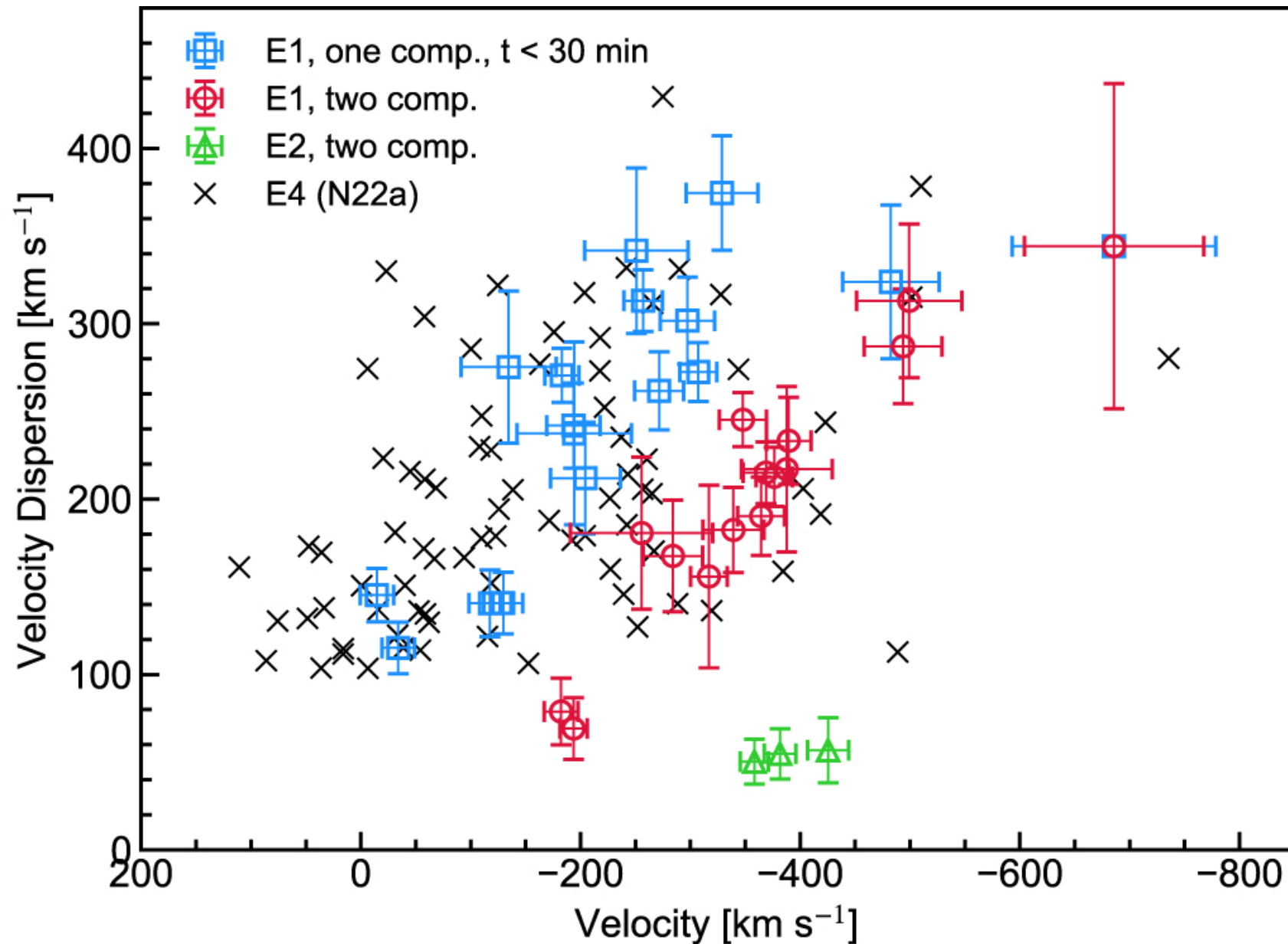
Figure 12. from Kosuke Namekata et al 2024 Astrophys. J. 961 doi:10.3847/1538-4357/ad0b7c https://dx.doi.org/10.3847/1538-4357/ad0b7c © 2024. The Author(s). Published by the American Astronomical Society.
