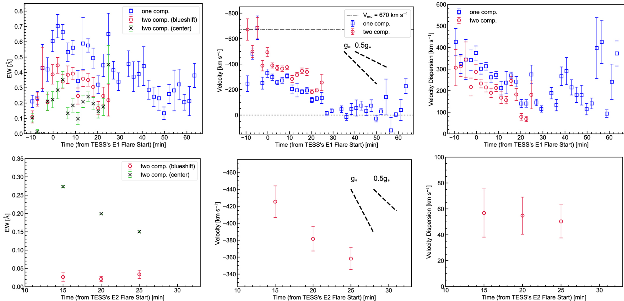
Figure 11. from Kosuke Namekata et al 2024 Astrophys. J. 961 doi:10.3847/1538-4357/ad0b7c https://dx.doi.org/10.3847/1538-4357/ad0b7c © 2024. The Author(s). Published by the American Astronomical Society.
