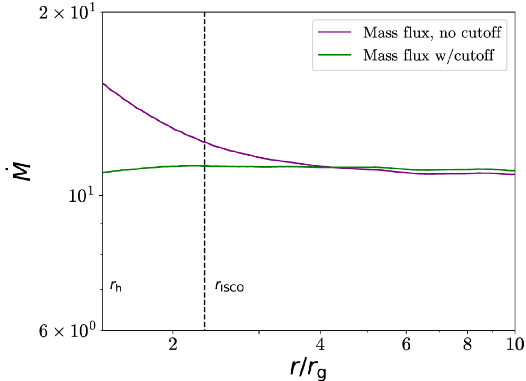
Figure 9. from Beverly Lowell et al 2024 Astrophys. J. 960 doi:10.3847/1538-4357/ad09af https://dx.doi.org/10.3847/1538-4357/ad09af © 2023. The Author(s). Published by the American Astronomical Society.
