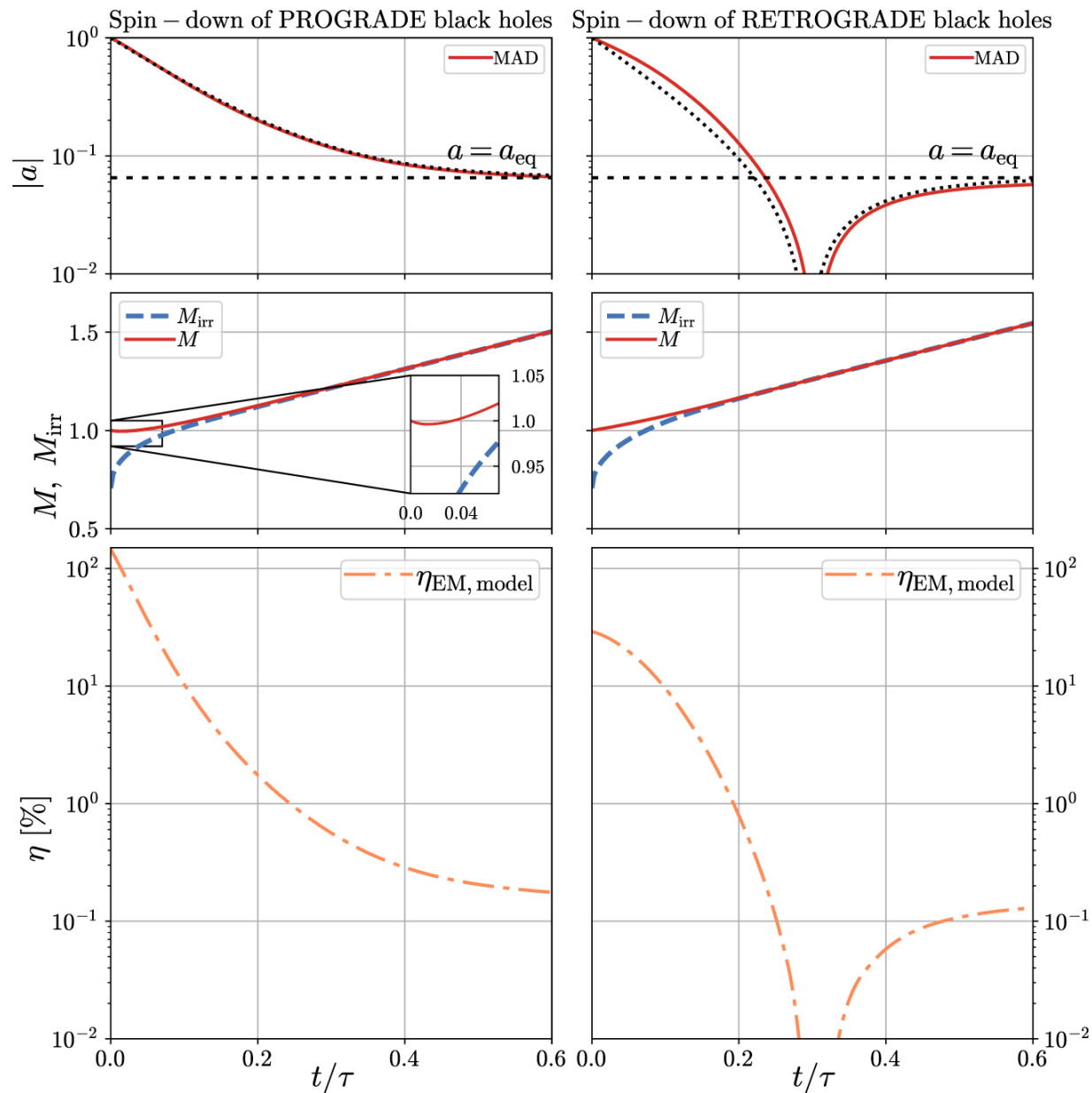
Figure 7. from Beverly Lowell et al 2024 Astrophys. J. 960 doi:10.3847/1538-4357/ad09af https://dx.doi.org/10.3847/1538-4357/ad09af © 2023. The Author(s). Published by the American Astronomical Society.
