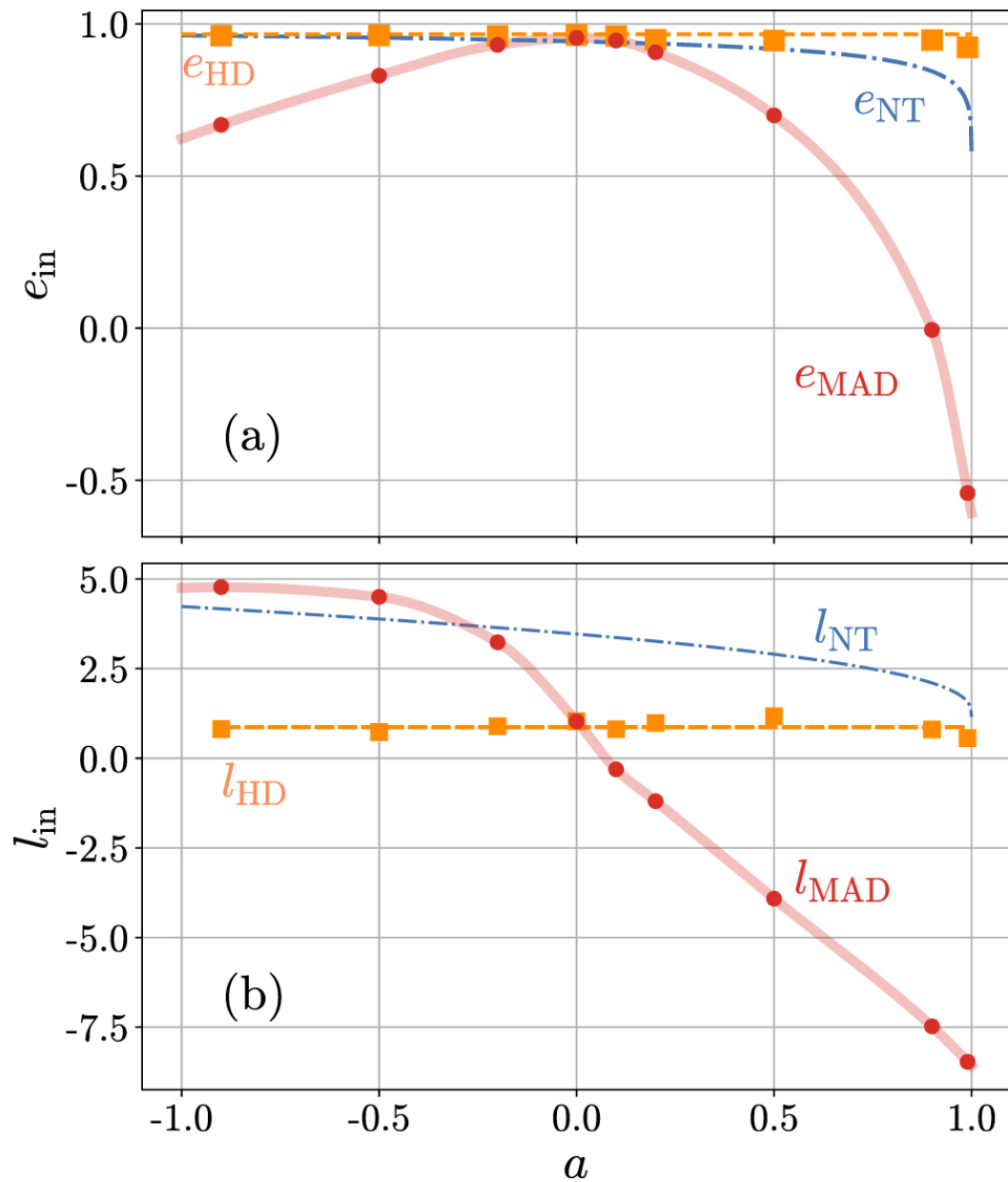
Figure 4. from Beverly Lowell et al 2024 Astrophys. J. 960 doi:10.3847/1538-4357/ad09af https://dx.doi.org/10.3847/1538-4357/ad09af © 2023. The Author(s). Published by the American Astronomical Society.
