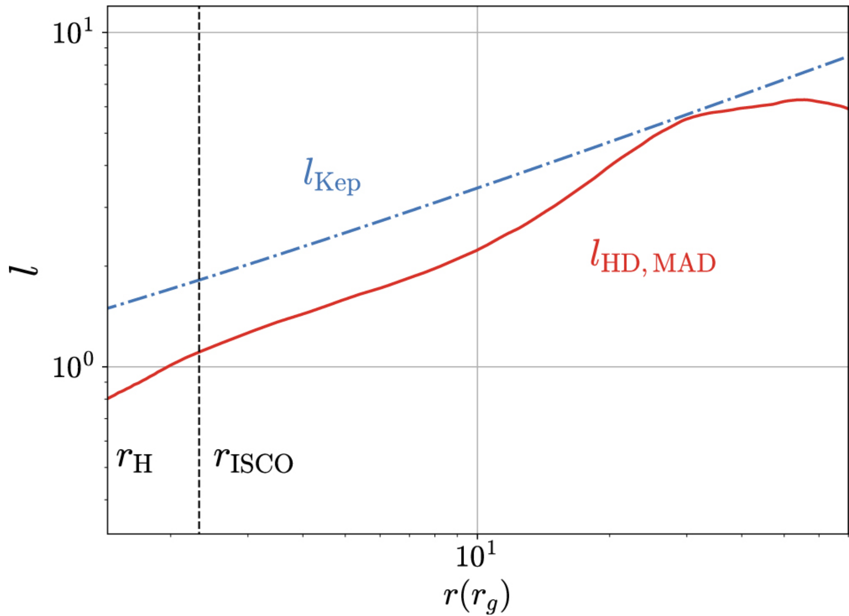
Figure 1. from Beverly Lowell et al 2024 Astrophys. J. 960 doi:10.3847/1538-4357/ad09af https://dx.doi.org/10.3847/1538-4357/ad09af © 2023. The Author(s). Published by the American Astronomical Society.
