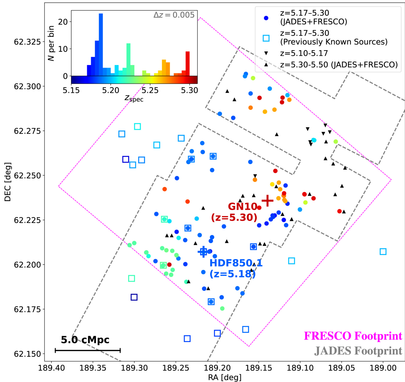
Figure 9. from Fengwu Sun et al 2024 Astrophys. J. 961 doi:10.3847/1538-4357/ad07e3 https://dx.doi.org/10.3847/1538-4357/ad07e3 © 2024. The Author(s). Published by the American Astronomical Society.
