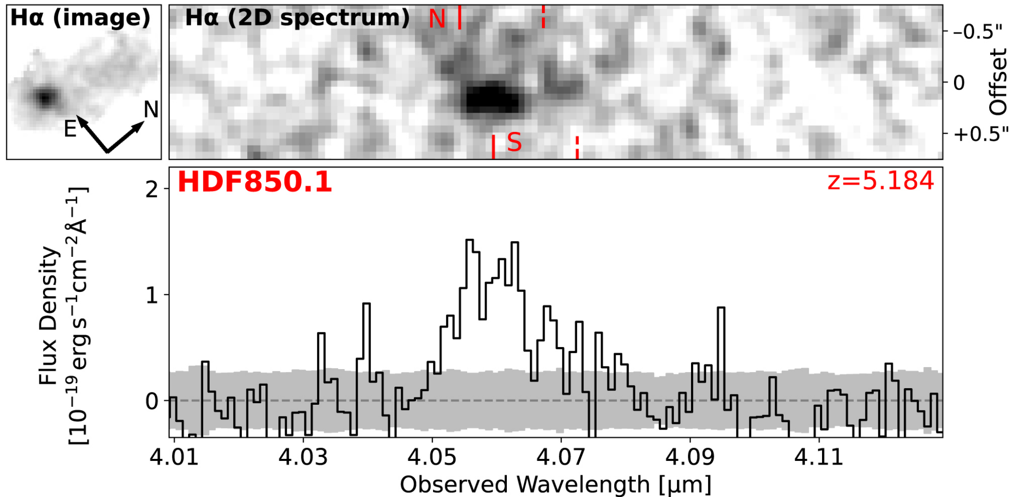
Figure 6. from Fengwu Sun et al 2024 Astrophys. J. 961 doi:10.3847/1538-4357/ad07e3 https://dx.doi.org/10.3847/1538-4357/ad07e3 © 2024. The Author(s). Published by the American Astronomical Society.
