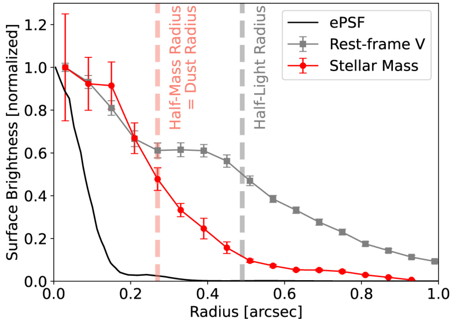
Figure 5. from Fengwu Sun et al 2024 Astrophys. J. 961 doi:10.3847/1538-4357/ad07e3 https://dx.doi.org/10.3847/1538-4357/ad07e3 © 2024. The Author(s). Published by the American Astronomical Society.
