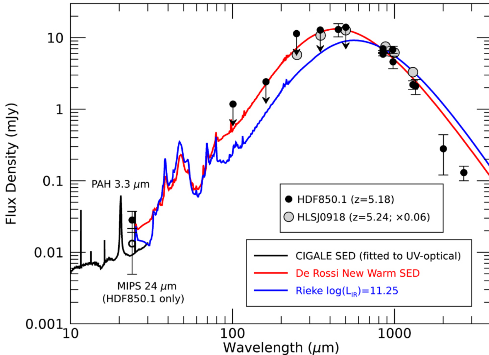
Figure 4. from Fengwu Sun et al 2024 Astrophys. J. 961 doi:10.3847/1538-4357/ad07e3 https://dx.doi.org/10.3847/1538-4357/ad07e3 © 2024. The Author(s). Published by the American Astronomical Society.
