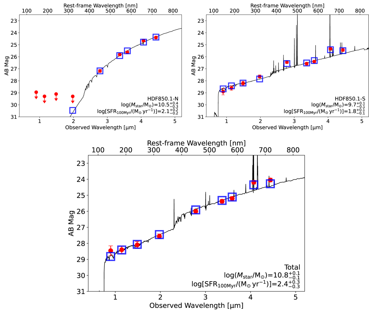
Figure 3. from Fengwu Sun et al 2024 Astrophys. J. 961 doi:10.3847/1538-4357/ad07e3 https://dx.doi.org/10.3847/1538-4357/ad07e3 © 2024. The Author(s). Published by the American Astronomical Society.
