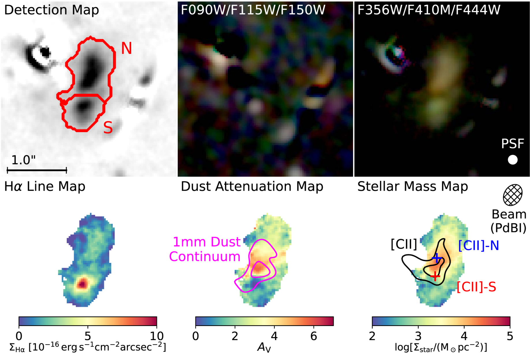
Figure 2. from Fengwu Sun et al 2024 Astrophys. J. 961 doi:10.3847/1538-4357/ad07e3 https://dx.doi.org/10.3847/1538-4357/ad07e3 © 2024. The Author(s). Published by the American Astronomical Society.
