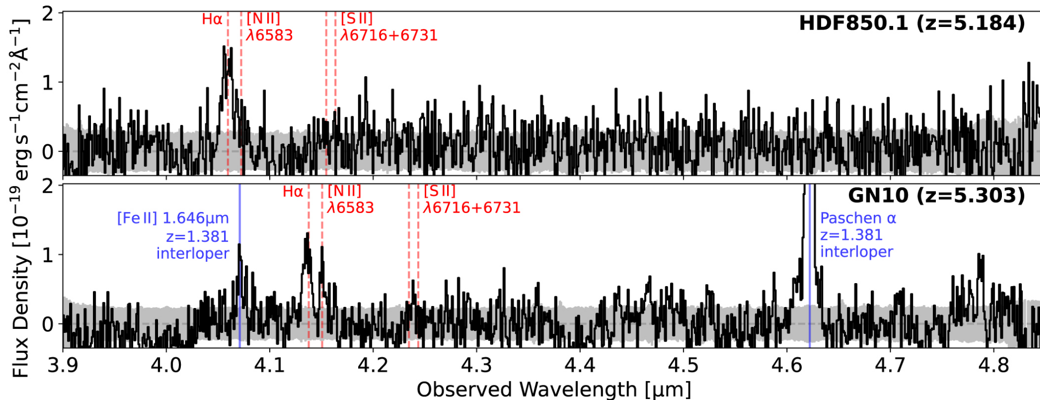
Figure A3. from Fengwu Sun et al 2024 Astrophys. J. 961 doi:10.3847/1538-4357/ad07e3 https://dx.doi.org/10.3847/1538-4357/ad07e3 © 2024. The Author(s). Published by the American Astronomical Society.
