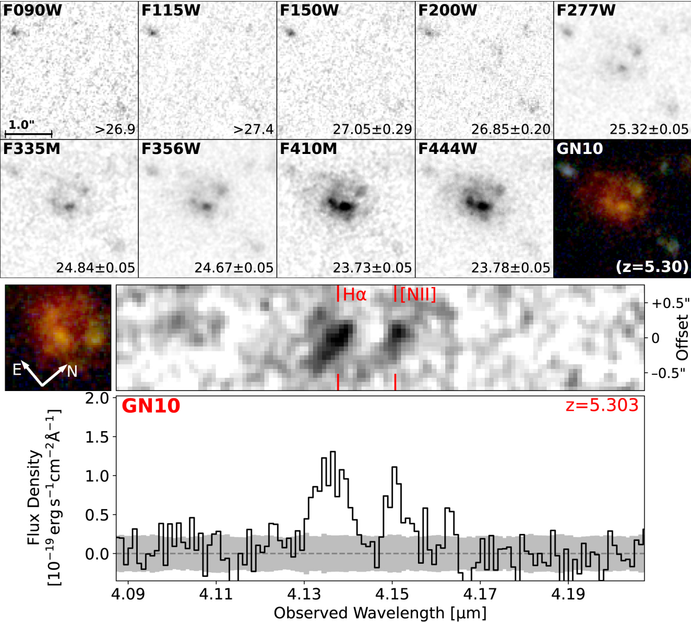
Figure A2. from Fengwu Sun et al 2024 Astrophys. J. 961 doi:10.3847/1538-4357/ad07e3 https://dx.doi.org/10.3847/1538-4357/ad07e3 © 2024. The Author(s). Published by the American Astronomical Society.
