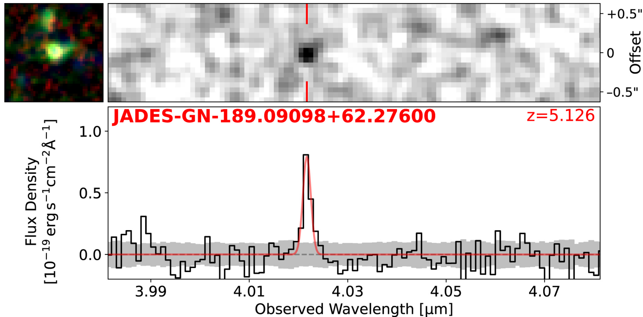
Figure A1. NIRCam images, 2D and 1D grism spectra of 140 spectroscopically confirmed galaxies at z = 5.1\text{--}5.5 . from Fengwu Sun et al 2024 Astrophys. J. 961 doi:10.3847/1538-4357/ad07e3 https://dx.doi.org/10.3847/1538-4357/ad07e3 © 2024. The Author(s). Published by the American Astronomical Society.
