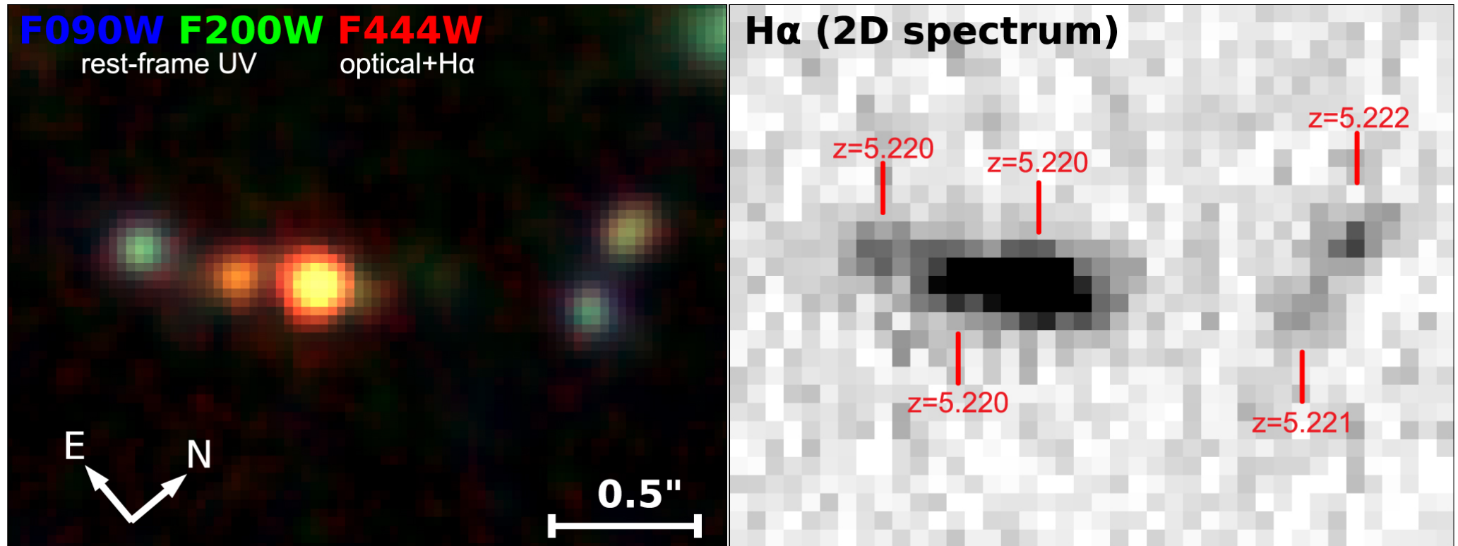
Figure 10. from Fengwu Sun et al 2024 Astrophys. J. 961 doi:10.3847/1538-4357/ad07e3 https://dx.doi.org/10.3847/1538-4357/ad07e3 © 2024. The Author(s). Published by the American Astronomical Society.
