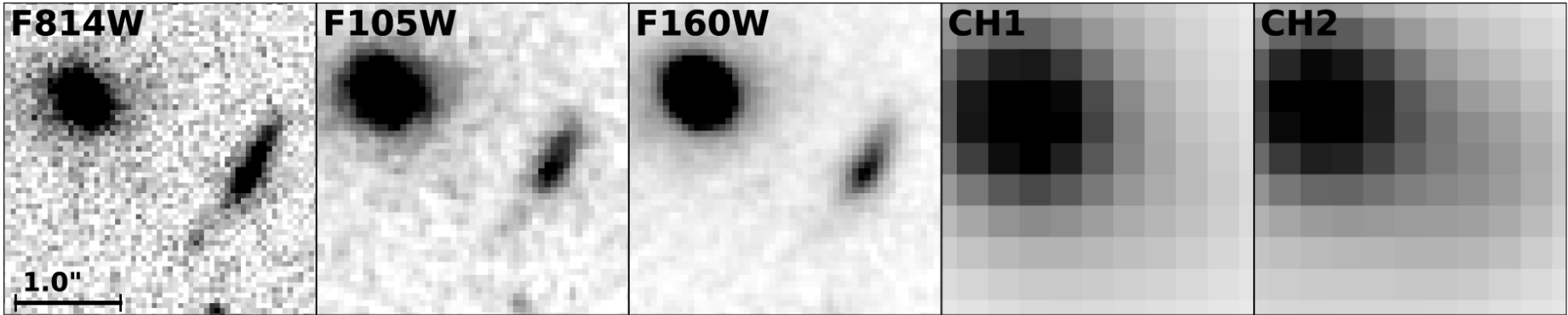
Figure 1. from Fengwu Sun et al 2024 Astrophys. J. 961 doi:10.3847/1538-4357/ad07e3 https://dx.doi.org/10.3847/1538-4357/ad07e3 © 2024. The Author(s). Published by the American Astronomical Society.
