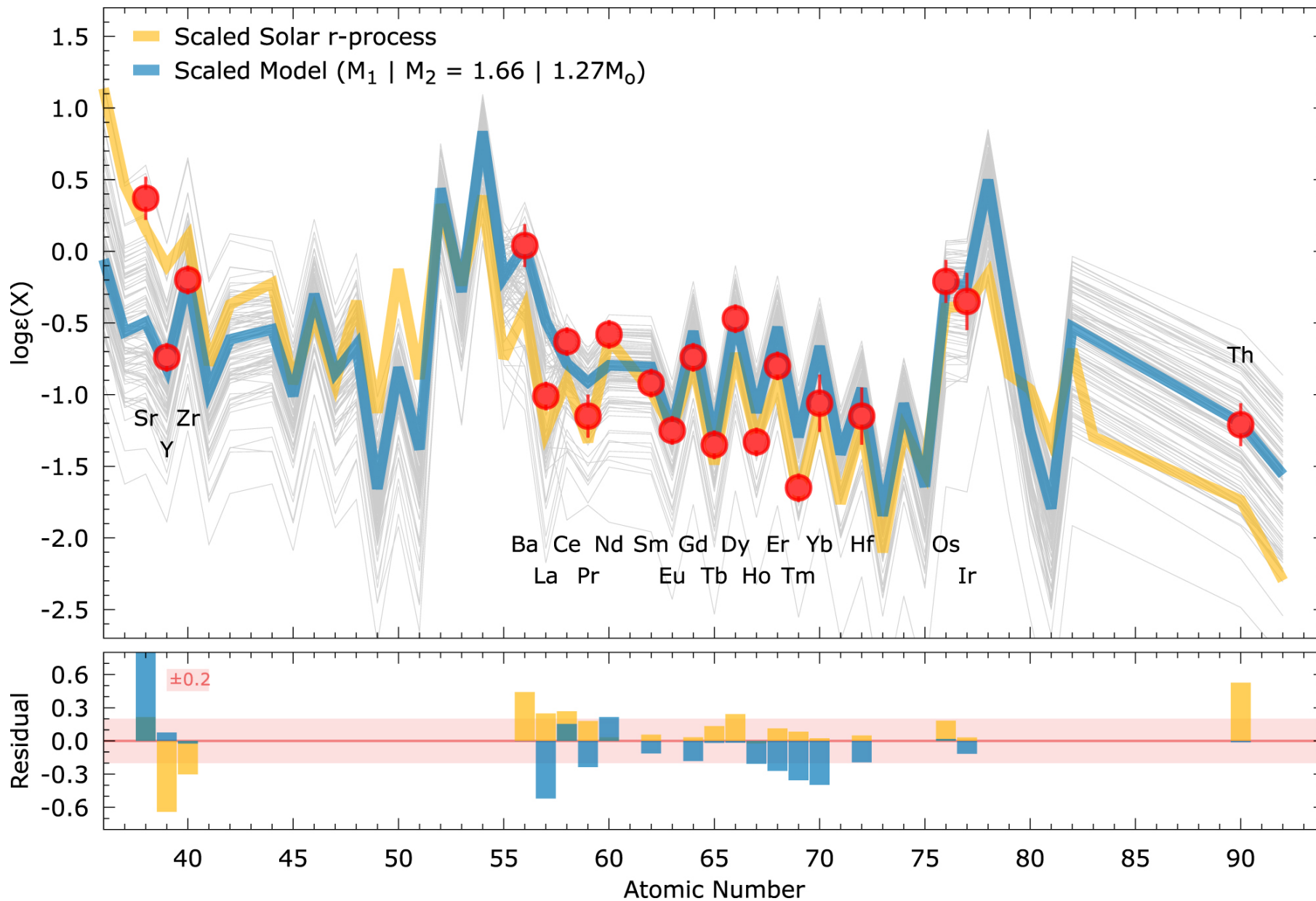
Figure 9. from Vinicius M. Placco et al 2023 Astrophys. J. 959 doi:10.3847/1538-4357/ad077e https://dx.doi.org/10.3847/1538-4357/ad077e © 2023. The Author(s). Published by the American Astronomical Society.
