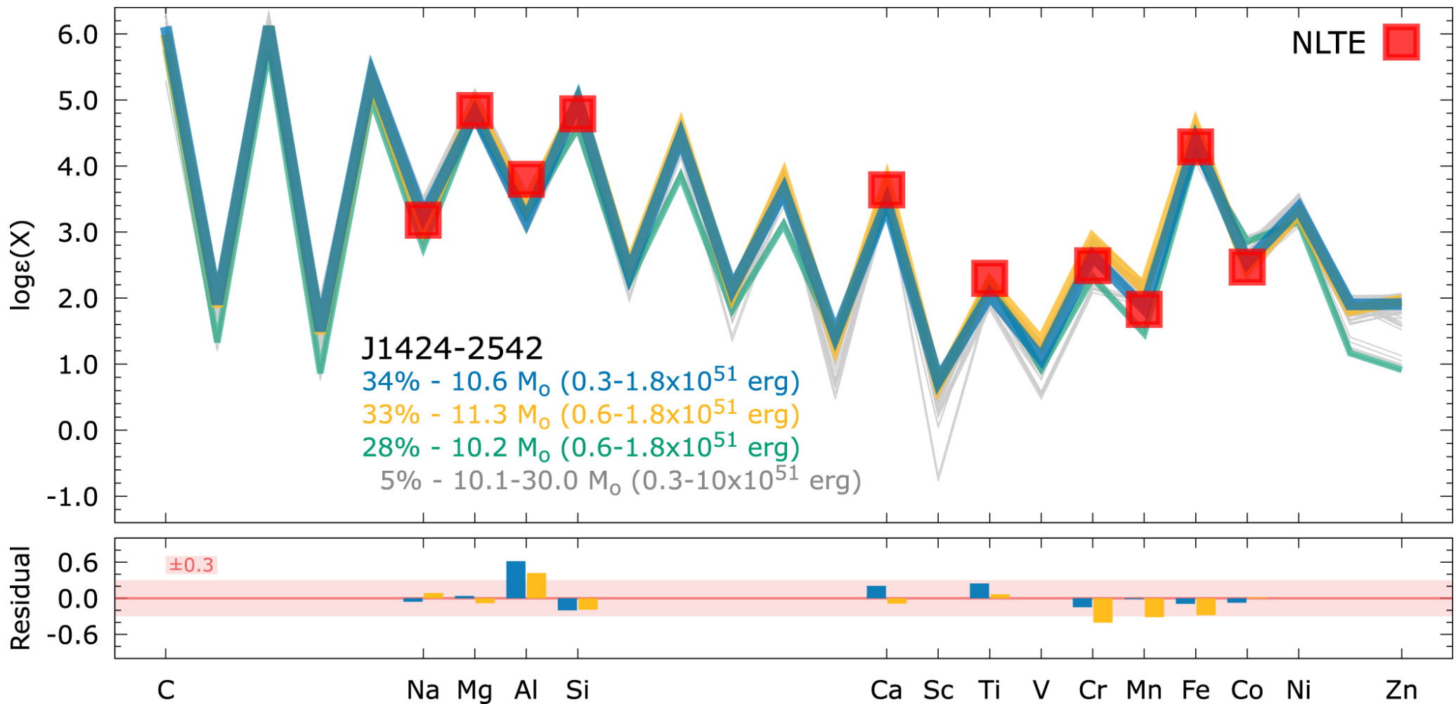
Figure 6. from Vinicius M. Placco et al 2023 Astrophys. J. 959 doi:10.3847/1538-4357/ad077e https://dx.doi.org/10.3847/1538-4357/ad077e © 2023. The Author(s). Published by the American Astronomical Society.
