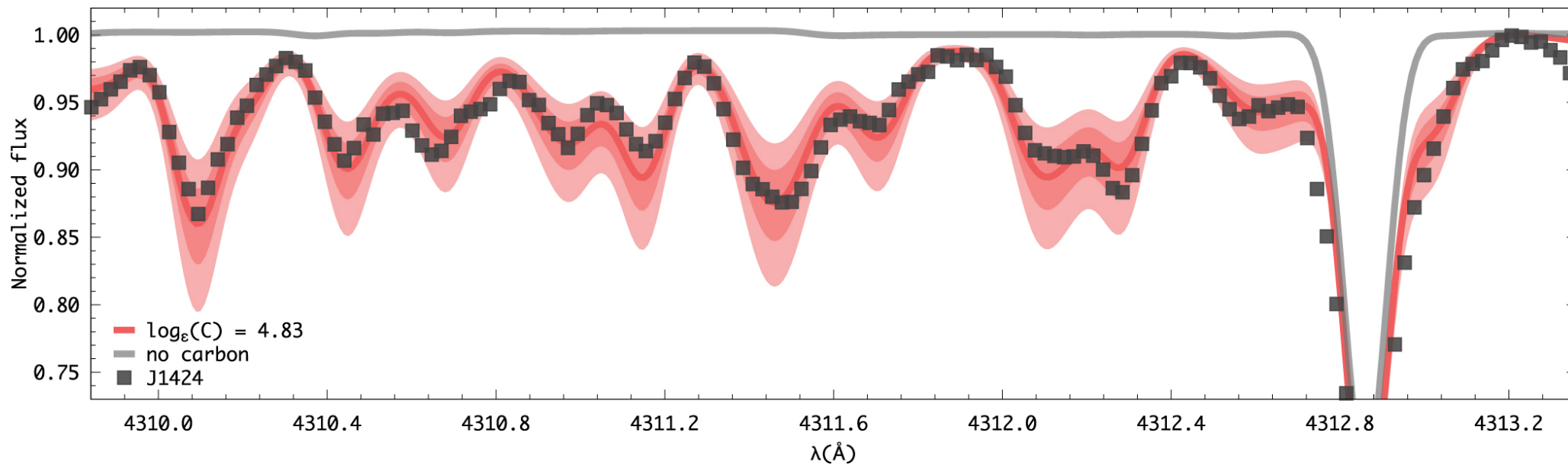
Figure 2. from Vinicius M. Placco et al 2023 Astrophys. J. 959 doi:10.3847/1538-4357/ad077e https://dx.doi.org/10.3847/1538-4357/ad077e © 2023. The Author(s). Published by the American Astronomical Society.
