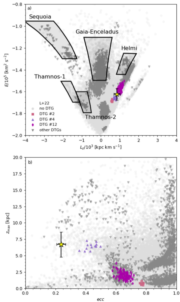
Figure 11. from Vinicius M. Placco et al 2023 Astrophys. J. 959 doi:10.3847/1538-4357/ad077e https://dx.doi.org/10.3847/1538-4357/ad077e © 2023. The Author(s). Published by the American Astronomical Society.
