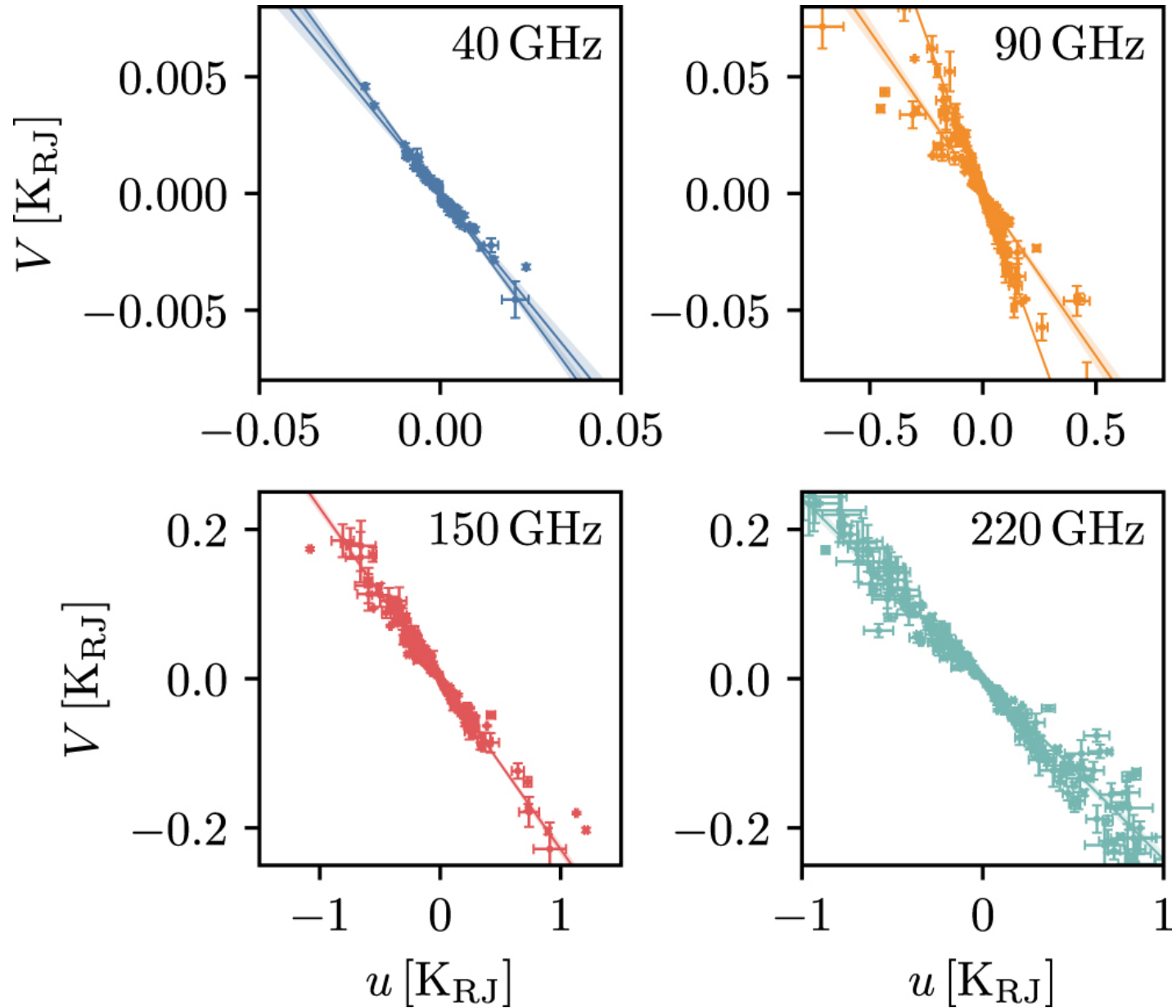
Figure 8. from Yunyang Li et al 2023 Astrophys. J. 958 doi:10.3847/1538-4357/ad0233 https://dx.doi.org/10.3847/1538-4357/ad0233 © 2023. The Author(s). Published by the American Astronomical Society.
