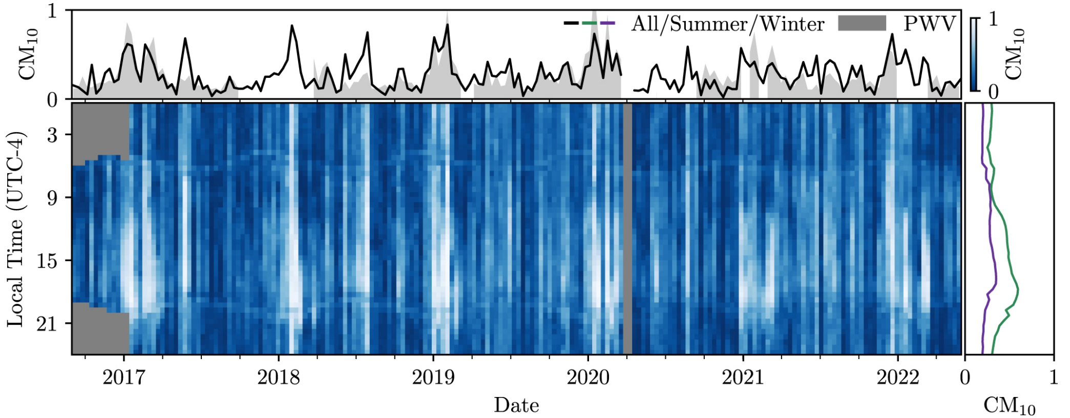
Figure 6. from Yunyang Li et al 2023 Astrophys. J. 958 doi:10.3847/1538-4357/ad0233 https://dx.doi.org/10.3847/1538-4357/ad0233 © 2023. The Author(s). Published by the American Astronomical Society.
