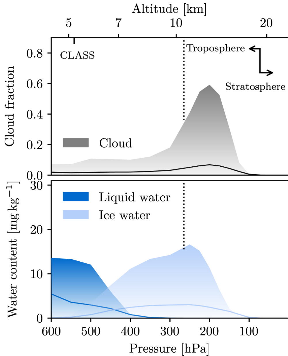
Figure 2. from Yunyang Li et al 2023 Astrophys. J. 958 doi:10.3847/1538-4357/ad0233 https://dx.doi.org/10.3847/1538-4357/ad0233 © 2023. The Author(s). Published by the American Astronomical Society.
