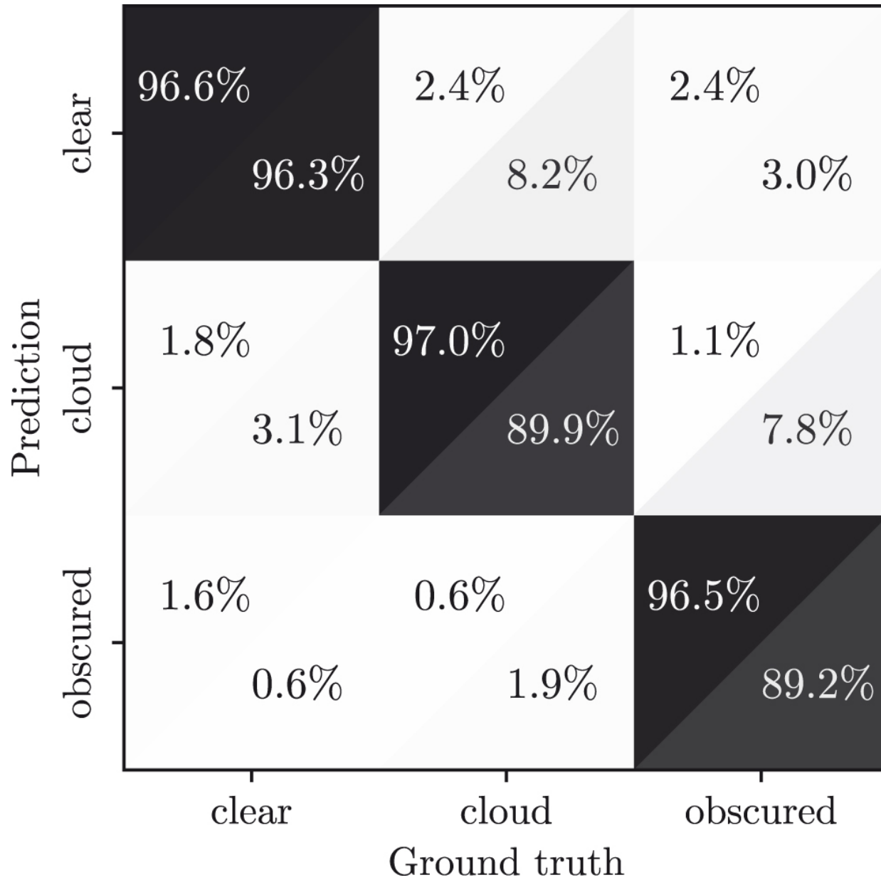
Figure 14. from Yunyang Li et al 2023 Astrophys. J. 958 doi:10.3847/1538-4357/ad0233 https://dx.doi.org/10.3847/1538-4357/ad0233 © 2023. The Author(s). Published by the American Astronomical Society.
