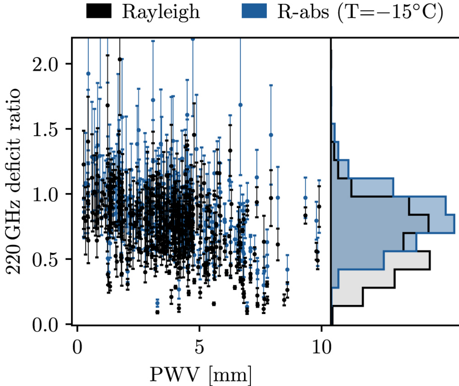
Figure 13. from Yunyang Li et al 2023 Astrophys. J. 958 doi:10.3847/1538-4357/ad0233 https://dx.doi.org/10.3847/1538-4357/ad0233 © 2023. The Author(s). Published by the American Astronomical Society.
