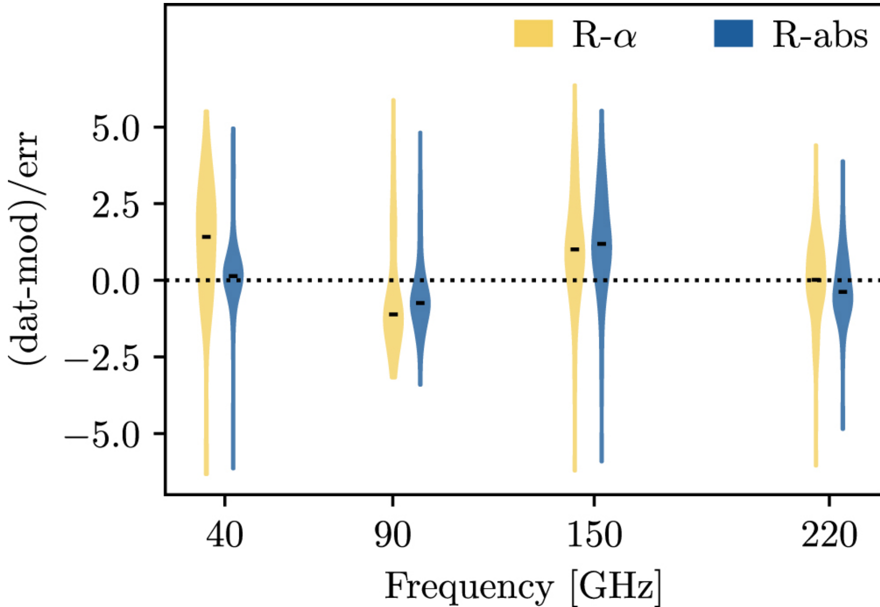
Figure 12. from Yunyang Li et al 2023 Astrophys. J. 958 doi:10.3847/1538-4357/ad0233 https://dx.doi.org/10.3847/1538-4357/ad0233 © 2023. The Author(s). Published by the American Astronomical Society.
