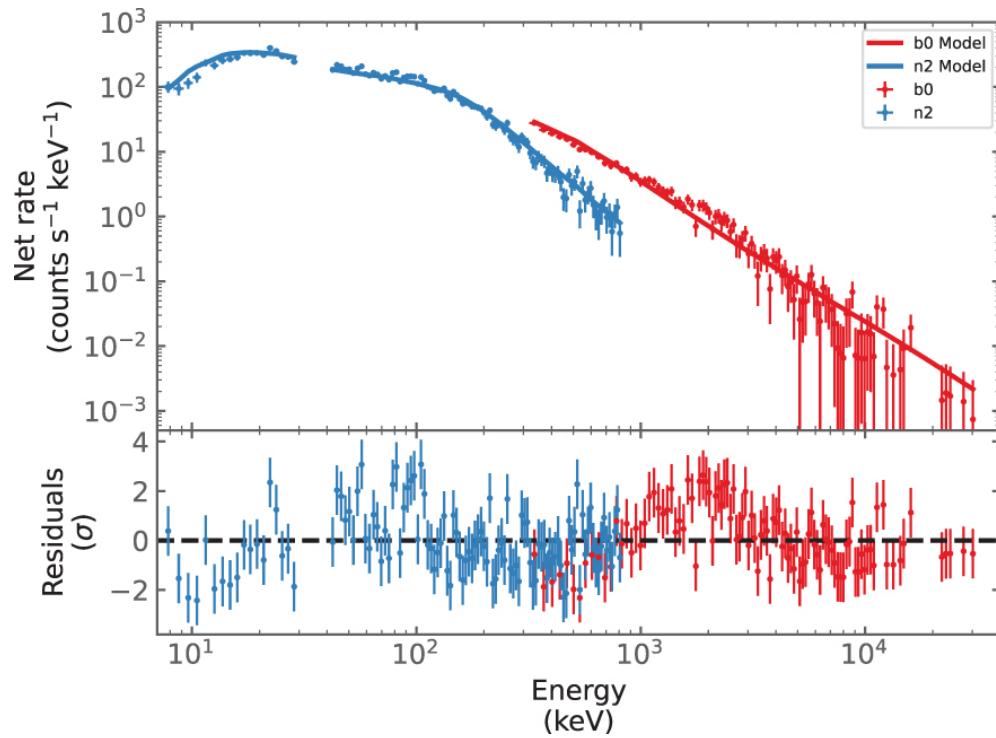
Figure 4. from Li Zhou et al 2023 Astrophys. J. 957 doi:10.3847/1538-4357/acfedc https://dx.doi.org/10.3847/1538-4357/acfedc © 2023. The Author(s). Published by the American Astronomical Society.
