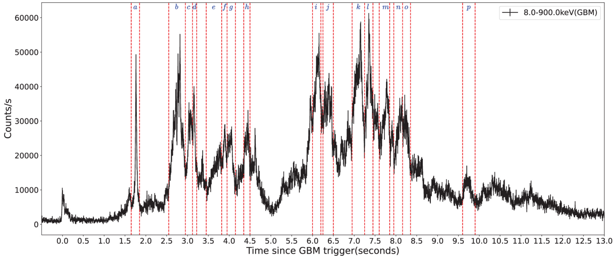
Figure 3. from Li Zhou et al 2023 Astrophys. J. 957 doi:10.3847/1538-4357/acfedc https://dx.doi.org/10.3847/1538-4357/acfedc © 2023. The Author(s). Published by the American Astronomical Society.
