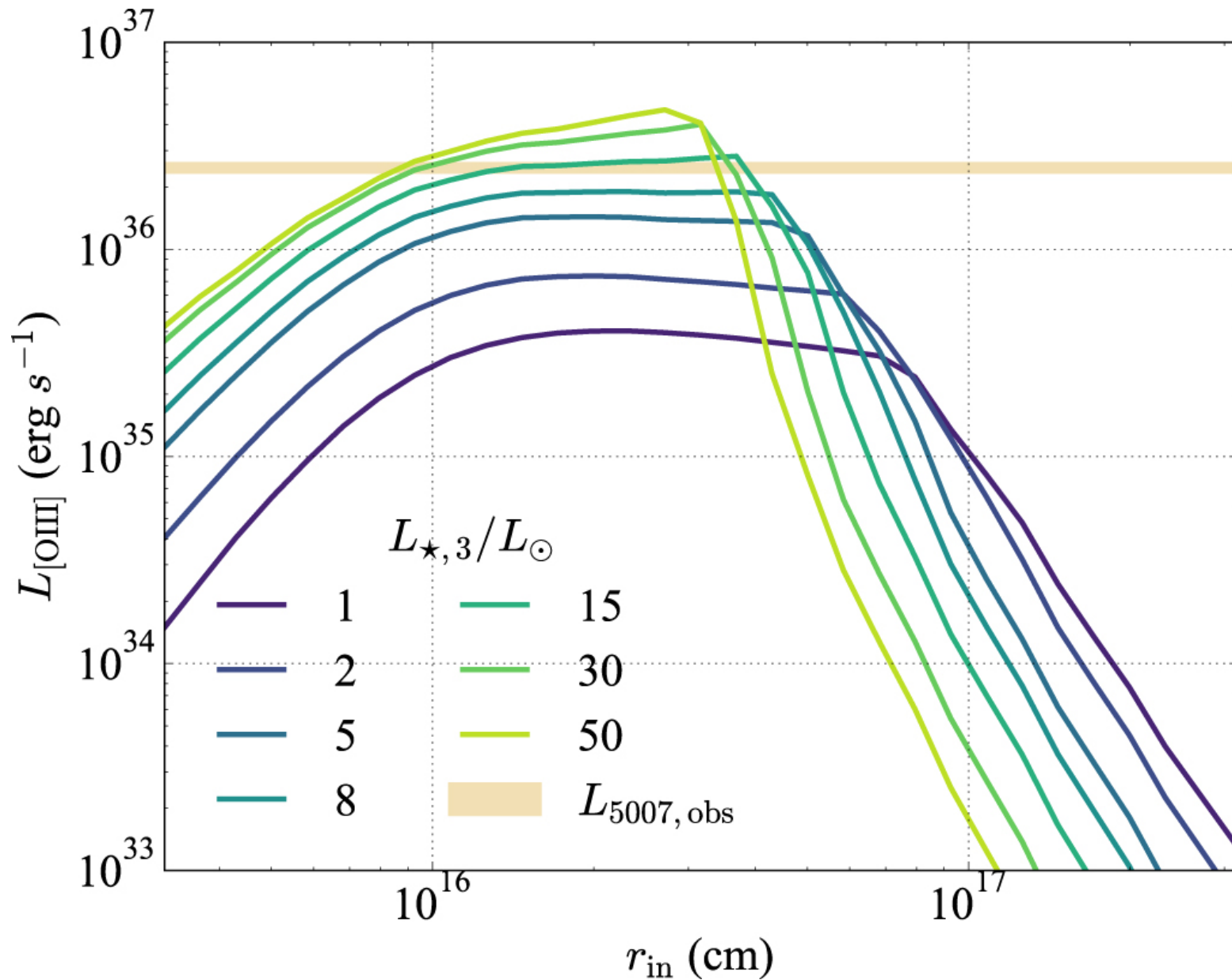
Figure 1. from Philippe Z. Yao and Eliot Quataert 2023 Astrophys. J. 957 doi:10.3847/1538-4357/acfed9 https://dx.doi.org/10.3847/1538-4357/acfed9 © 2023. The Author(s). Published by the American Astronomical Society.
