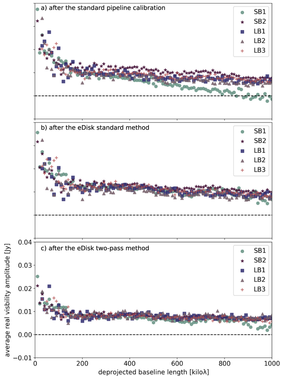
Figure 1. from Suchitra Narayanan et al 2023 Astrophys. J. 958 doi:10.3847/1538-4357/acfd24 https://dx.doi.org/10.3847/1538-4357/acfd24 © 2023. The Author(s). Published by the American Astronomical Society.
