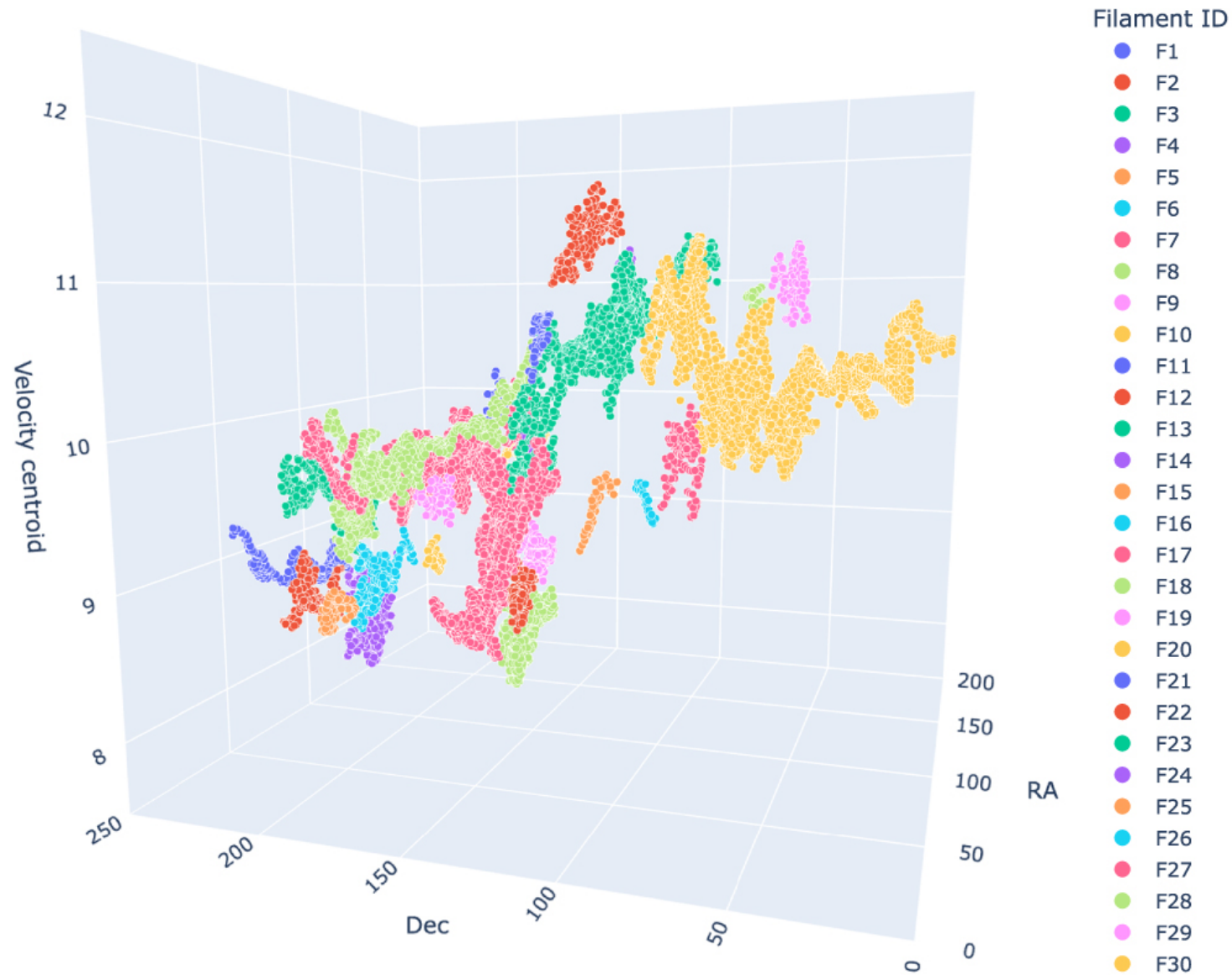
Figure 9. from Hyunju Yoo et al 2023 Astrophys. J. 957 doi:10.3847/1538-4357/acf8c2 https://dx.doi.org/10.3847/1538-4357/acf8c2 © 2023. The Author(s). Published by the American Astronomical Society.
